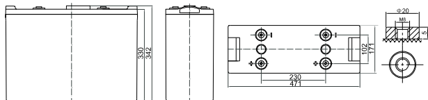
Terminal Dimensions
